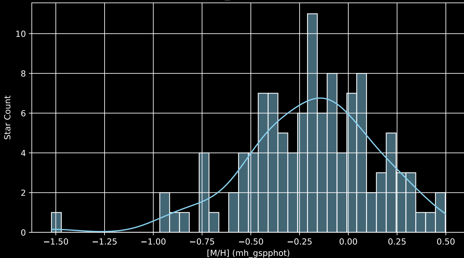
APOGEE DR17 Field: [279-36-O_TESS [M/H] (mh_gspphot) (n= 113)
