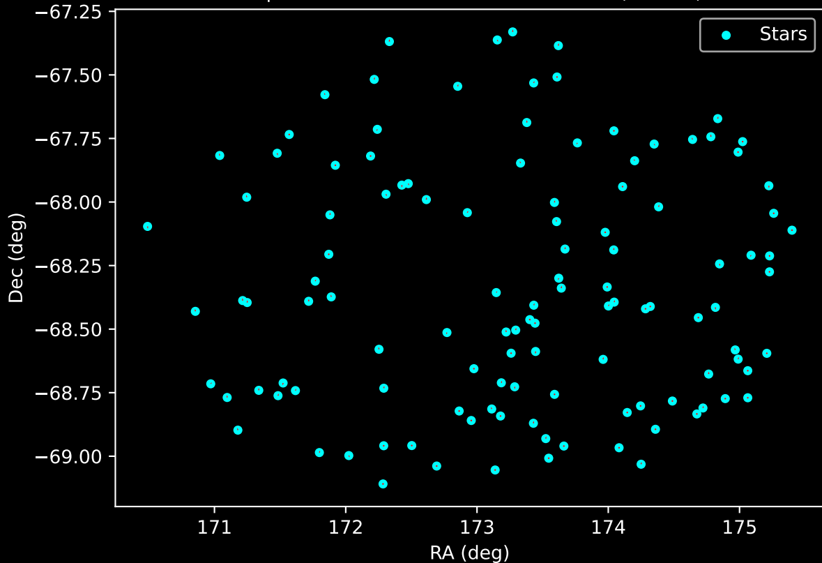
APOGEE DR17 Field: [279-36-O_TESS] Proper Motion Vectors for Gaia Star Field (n= 117)
