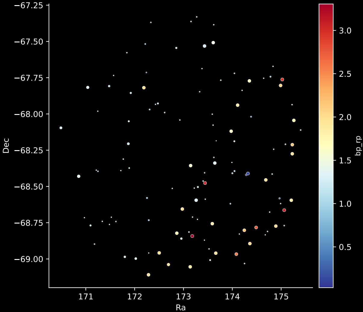
APOGEE DR17 Field: [279-36-O_TESS] Stars: 117
