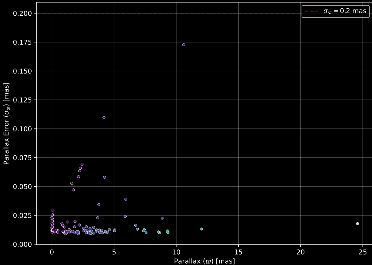
APOGEE DR17 Field: [279-36-O_TESS] Parallax Quality (n= 117)
