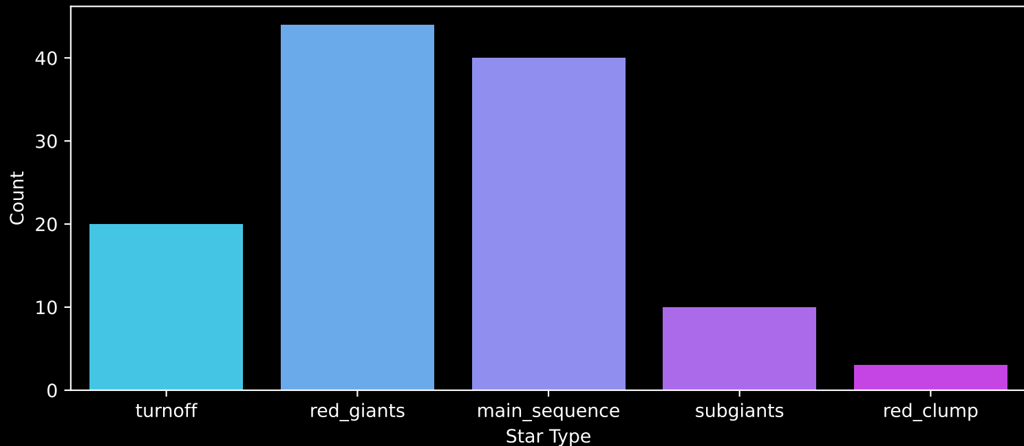
APOGEE DR17 Field: [279-36-O_TESS] Count plot of Star Type
