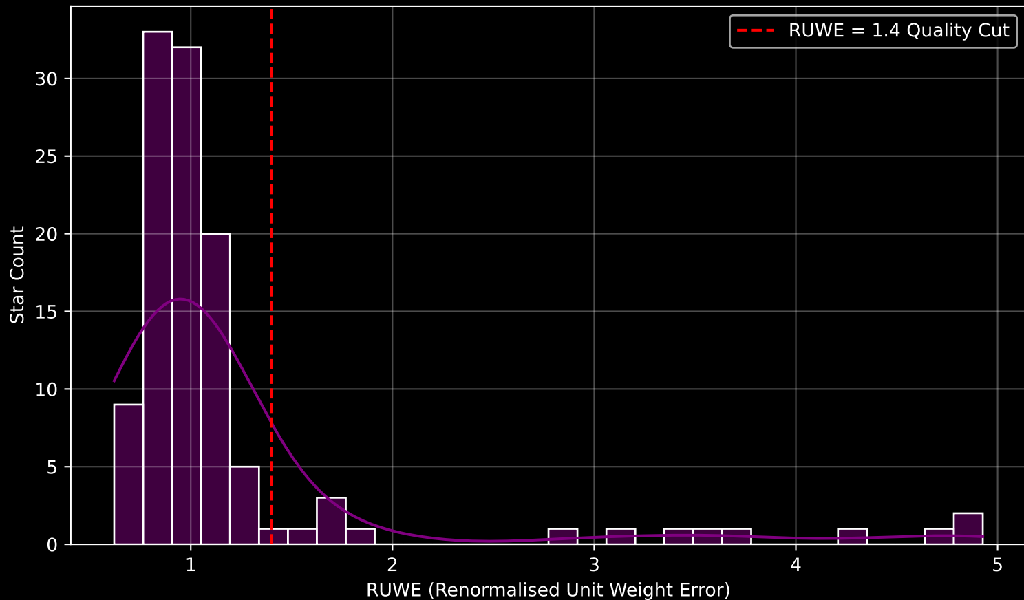
GAPOGEE DR17 Field [279-36-O_TESS] RUWE Distribution (n= 114)
