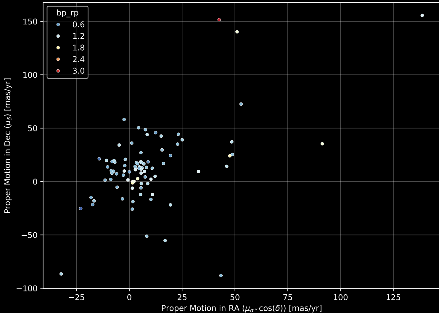
APOGEE DR17 Field: [279-36-O_TESS] Proper Motion Diagram (n= 117)
